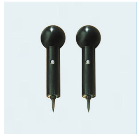
Electrode E16 for hard bldg materials and cement-based panels for - Ligno-VersaTec
