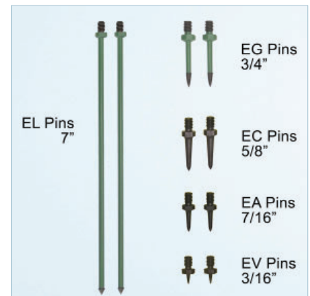
Selection of Pins for E16: EG, EL, EA, EC, EV
